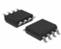
TC4431VOA Micrel / Microchip Technology IC MOSFET DRIVER 30V 1.5A 8SOIC
