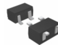
XC6109N44ANR-G Torex Semiconductor Ltd IC SUPERVISOR 4.4V SSOT24-4
