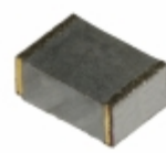
ECW-U4562V17 Panasonic Electronic Components CAP FILM 5600PF 5% 400VDC 1913
