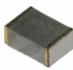
ECW-U4682V17 Panasonic Electronic Components CAP FILM 6800PF 5% 400VDC 1913
