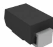
BY11-90-E3/TR3 Vishay / Semiconductor - Diodes Division DIODE SCHOTTKY 90V 1.5A DO214AC
