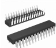
PIC16C57C-04I/SP Microchip Technology IC MCU 8BIT 3KB OTP 28SDIP
