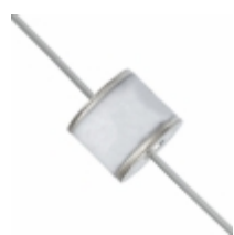
CG21000LTR Littelfuse Inc. GDT 1000V 10KA THROUGH HOLE
