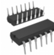
MCP4241-104E/P Microchip Technology IC DGTL POT DL 100K 2CH 14-DIP
