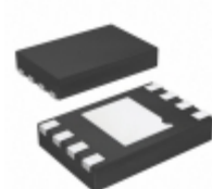
BR93G86NUX-3BTTR Rohm Semiconductor IC EEPROM 16KBIT 3MHZ 8VSON
