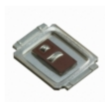
IRF6709S2TRPBF Infineon Technologies MOSFET N-CH 25V 12A DIRECTFET-S1
