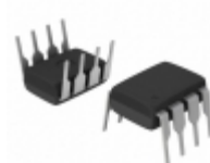
AT24C08-10PC-1.8 Microchip Technology IC EEPROM 8KBIT 400KHZ 8DIP
