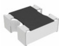
EXB-24AB3CR8X Panasonic Electronic Components ATTENUATOR 3DB 100 OHM 0404 SMD
