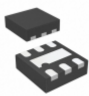
MIC5370-M4YMT-TR Microchip Technology IC REG LDO 2.8V/1.2V 0.15A 6TMLF
