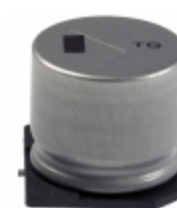
EEV-TG1C332M Panasonic Electronic Components CAP ALUM 3300UF 20% 16V SMD
