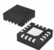
MCP4651T-502E/ML Microchip Technology IC DGTL POT 5K 257TAPS 16-QFN
