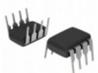
REF02DN8#PBF ADI (Analog Devices, Inc.) IC VREF SERIES 5V 8DIP
