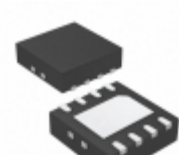
PIC12C672T-04I/MF Microchip Technology IC MCU 8BIT 3.5KB OTP 8DFNS
