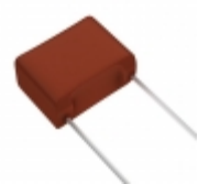
ECW-F2125HA Panasonic Electronic Components CAP FILM 1.2UF 3% 250VDC RADIAL
