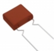
ECW-F2124JAQ Panasonic Electronic Components CAP FILM 0.12UF 5% 250VDC RADIAL
