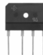
GSIB2080N-M3/45 Electro-Films (EFI) / Vishay BRIDGE RECT 20A 800V GSIB-5S
