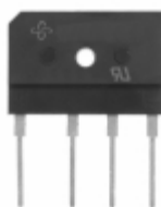
GSIB2080-E3/45 Electro-Films (EFI) / Vishay DIODE 20A 800V GSIB-5S
