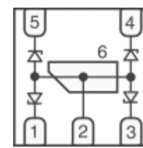
VESD09A4A-HS4-GS08 Vishay Semiconductor Diodes Division TVS DIODE 9VWM 23VC LLP10106L
