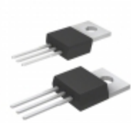
DHG40C600PB IXYS DIODE ARRAY GP 600V 20A TO220AB
