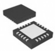
MCP4361T-503E/ML Microchip Technology IC DGTL POT QUAD 50K 20QFN
