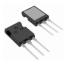
IXFX32N100P IXYS MOSFET N-CH 1000V 32A PLUS247
