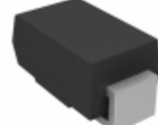
SMBZ5929B-E3/5B Vishay Semiconductor Diodes Division DIODE ZENER 15V 3W DO214AA
