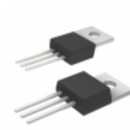
IXFP14N60P IXYS MOSFET N-CH 600V 14A TO-220
