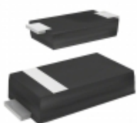
CZRA4750-HF Comchip Technology DIODE ZENER 27V 1W DO214AC
