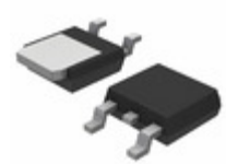
MJD350T4 ON Semiconductor TRANS PNP 300V 0.5A DPAK
