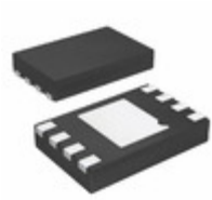
AT25320B-MAHL-E Micrel / Microchip Technology IC EEPROM 32K SPI 20MHZ 8UDFN
