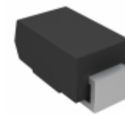
P4SMA33A-E3/61 Electro-Films (EFI) / Vishay TVS DIODE 28.2V 45.7V DO214AC
