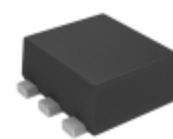
US6U37TR Rohm Semiconductor MOSFET N-CH 30V 1.5A TUMT6
