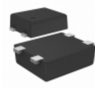
S-80152BLPF-JFDTFG SII Semiconductor Corporation IC VOLT DETECTOR 5.2V SNT-4A
