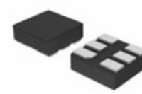
NLAS3157MX3TCG ON Semiconductor IC SWITCH SPDT 9.9 OHM ULLGA6
