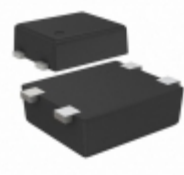
S-80131BLPF-JEQTG SII Semiconductor Corporation IC VOLT DETECTOR 3.1V SNT-4A
