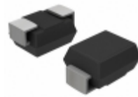
1SMB5917BT3 ON Semiconductor DIODE ZENER 4.7V 3W SMB
