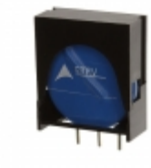
ETFV20K130E2 EPCOS (TDK) VARISTOR 205V 10KA RADIAL
