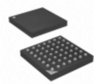
ATXMEGA32D4-CU Microchip Technology IC MCU 8BIT 32KB FLASH 49VFBGA
