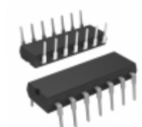
MCP4261-103E/P Microchip Technology IC DGTL POT 10K 2CH 14DIP
