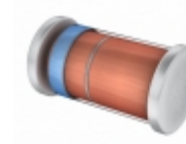
CLL4742A TR Central Semiconductor Corp DIODE ZENER 12V 1W MELF
