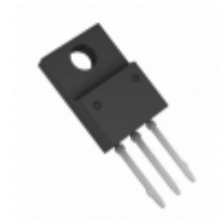
BA7806CP-E2 LAPIS Semiconductor IC REG LDO 6V 1A TO220CP-3
