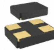
CX3225GB14745D0HPQZ1 AVX Corporation CRYSTAL 14.7456MHZ 8PF SMD
