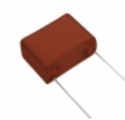
ECW-F2335HA Panasonic Electronic Components CAP FILM 3.3UF 3% 250VDC RADIAL
