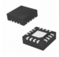
PL135-47QC-R Microchip Technology IC CLK BUFFER 1:4 40MHZ 16QFN
