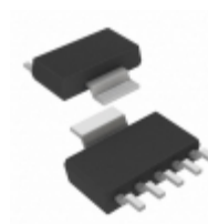
MCP1825T-ADJE/DC Microchip Technology IC REG LDO ADJ 0.5A SOT223-5
