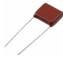
ECQ-E2155KF3 Panasonic Electronic Components CAP FILM 1.5UF 10% 250VDC RADIAL
