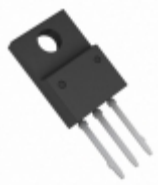
BA78M20CP-E2 Rohm Semiconductor IC REG LDO 20V 0.5A TO220CP-3
