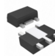
AP2112R5-1.2TRG1 Diodes Incorporated IC REG LDO 1.2V 0.6A SOT89-5
