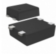
S-1000N20-I4T1G SII Semiconductor Corporation IC VOLT DETECT N-CH 20V SNT-4A
