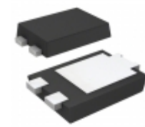
DXT2014P5-13 Diodes Incorporated TRANS PNP 140V 4A POWERDI5
