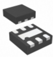
MIC94345-GYMT-T5 Microchip Technology IC REG LDO 1.8V 0.5A 6TDFN
