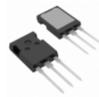
IXFX55N50F IXYS RF MOSFET N-CH 500V 55A PLUS247
