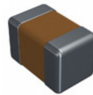
CDR31BP120BJWRAC Electro-Films (EFI) / Vishay CAP CER 12PF 100V BP 0805
